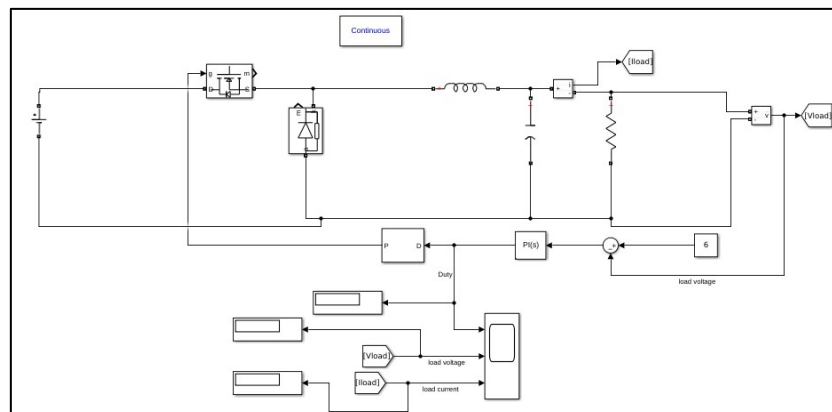
Fig.5. Buck converter schematic diagram with the PWM
